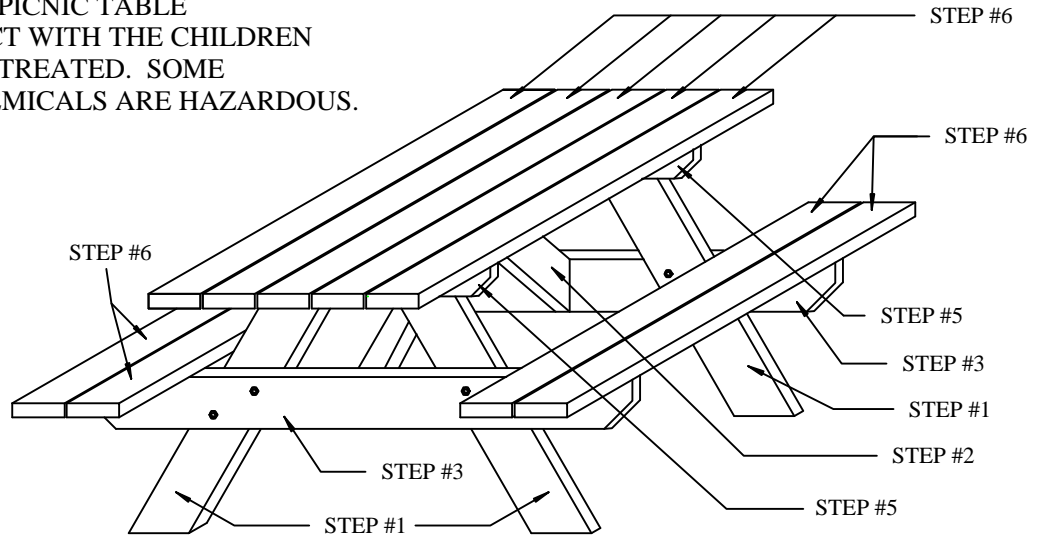
Figure #1 - Isometric Assembled Table
