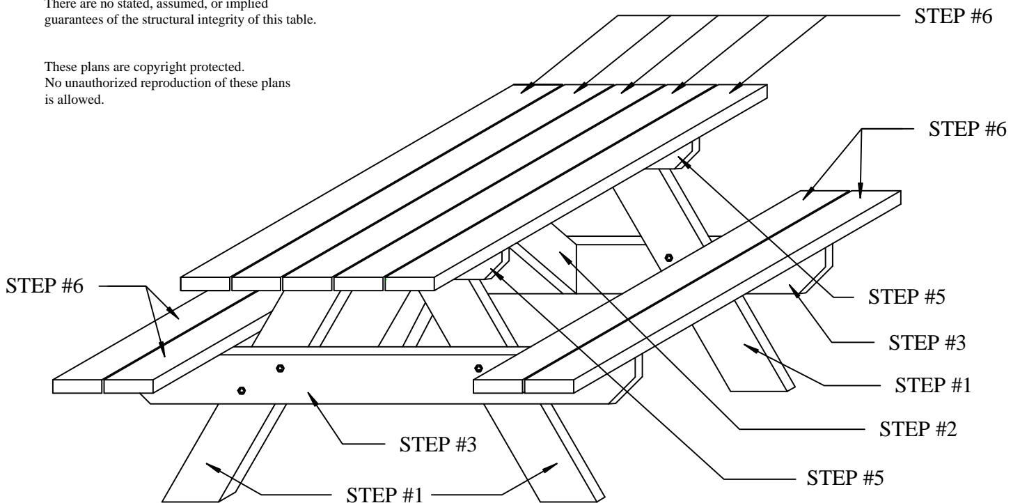
Figure #1 - Isometric Assembled Table
